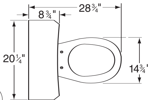
Specifications: Bowl — #21-377 Elongated Bowl Tank — #28-380 Seat not included
