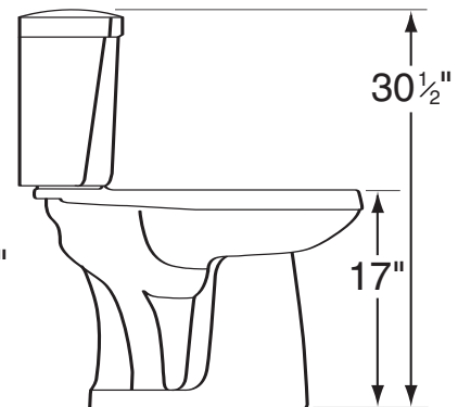
Specifications: Bowl — #21-377 Elongated Bowl Tank — #28-380 Seat not included
