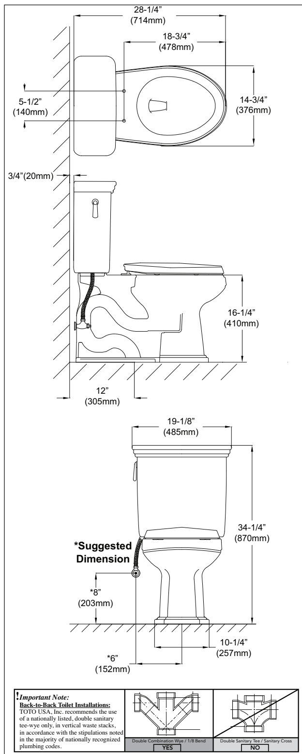
CST424SF(G) - Promenade Close Coupled Toilet
