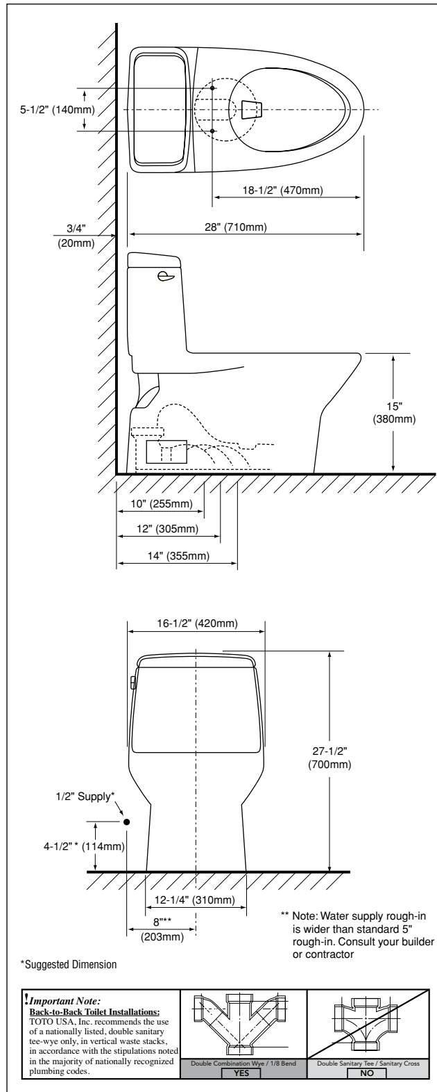
MS874114S(G) - Carlyle Toilet with SanaGloss and SoftClose Seat
